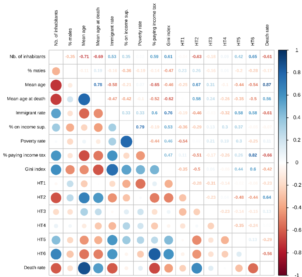
Figure 2. Correlation matrix.
